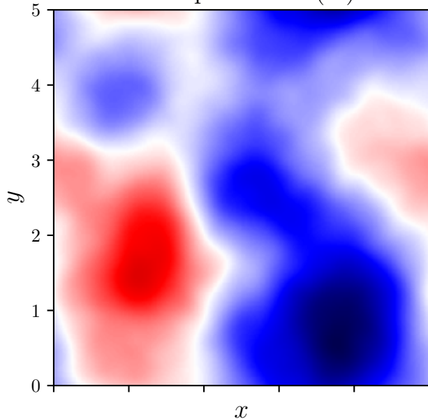
Final x displacement (m) id=0
